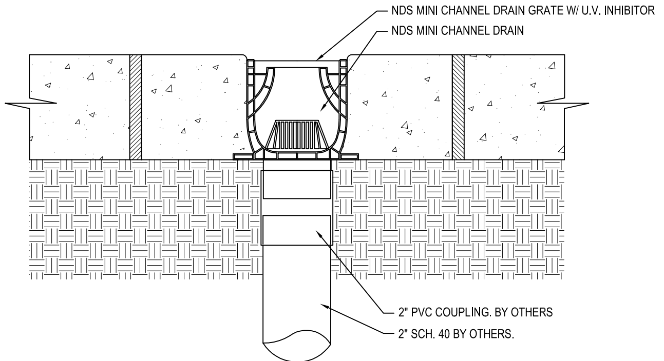
SECTION
